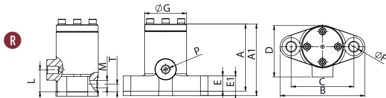
DIMENSIONAL SPECIFICATIONS
