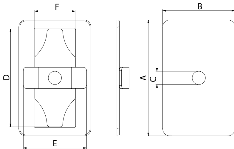
DIMENSIONAL SPECIFICATIONS
