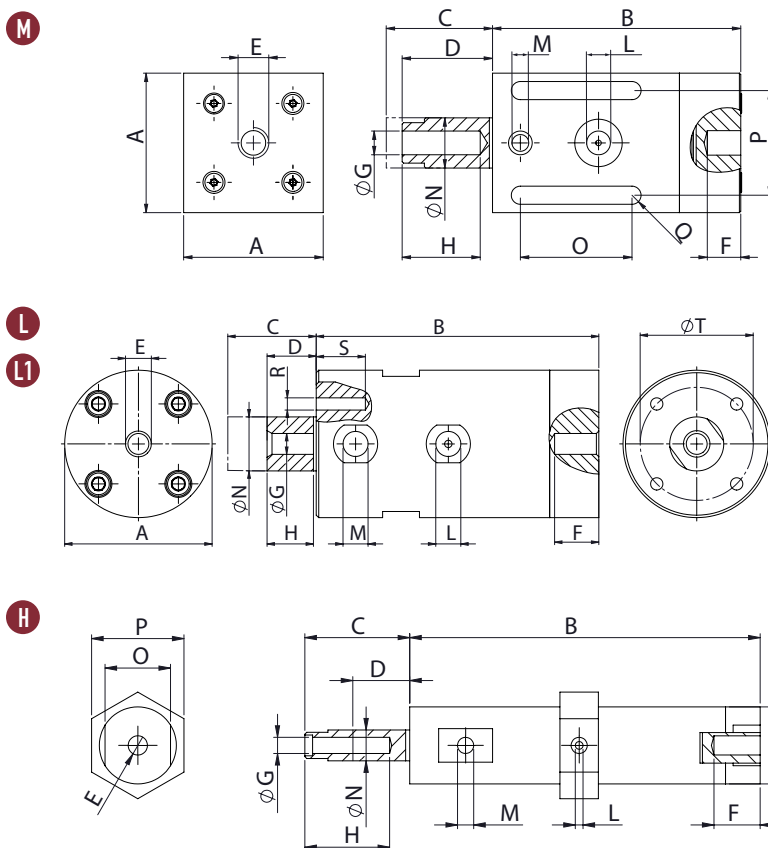
DIMENSIONAL SPECIFICATIONS
