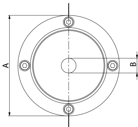
DIMENSIONAL SPECIFICATIONS
