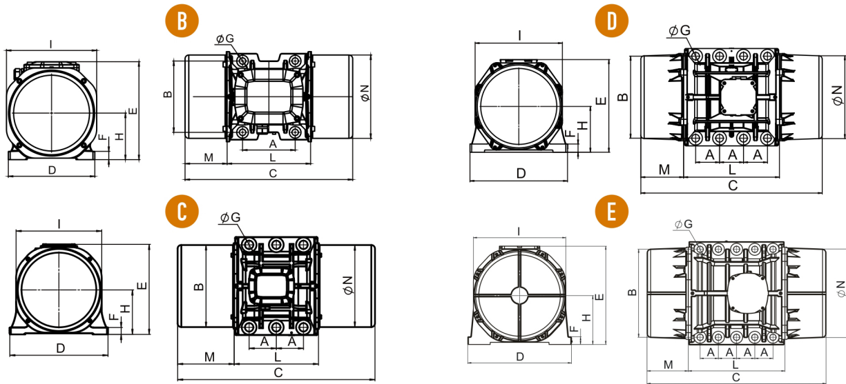
6 POLES - 1000 rpm
